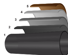
(1) Galvanized Pipe (2) Phosphate Adhesion Wash (3) Conversion Coating (4) UV Inhibitor (5) Powder Coating
